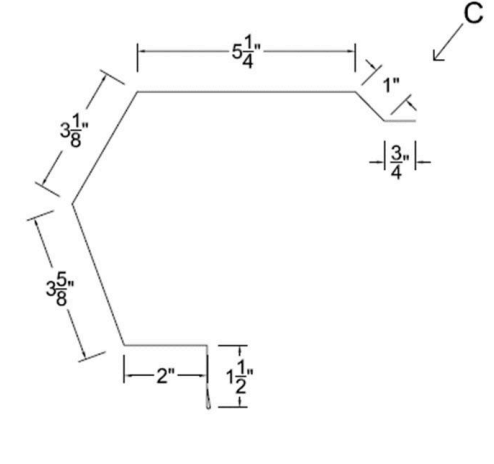
U Panel Sculptured Rake
