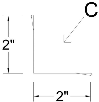
Inside Angle 2" x 2"
