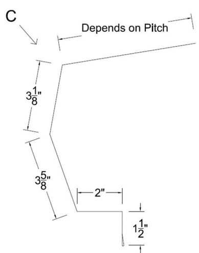
Peak Box Sculptured Rake
