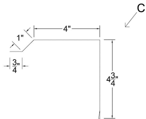
U Panel House Rake
