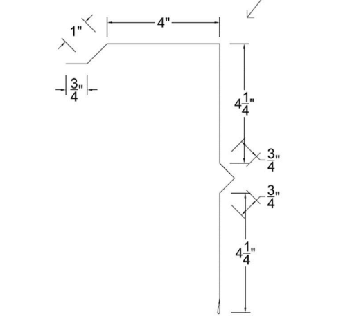
U Panel House Rake 9 1/2" Reveal
