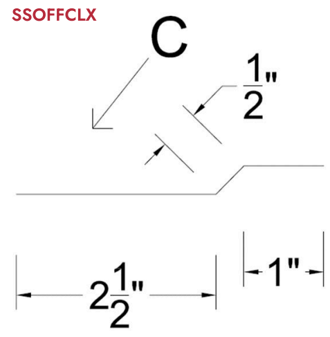
Standing Seam Offset Cleat
