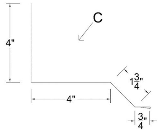
R Panel Rakewall
