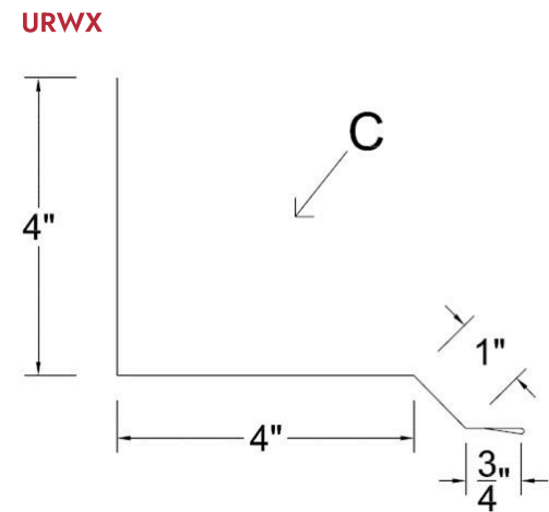
U Panel Rakewall
