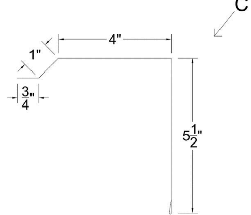
U Panel House Rake 5 1/2" Reveal
