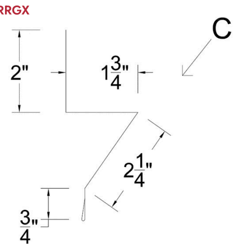
R Panel Rat Guard
