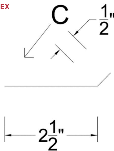
Standing Seam Cleat
