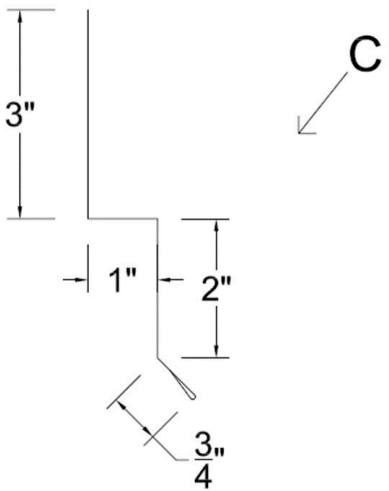
U Panel Wainscot
