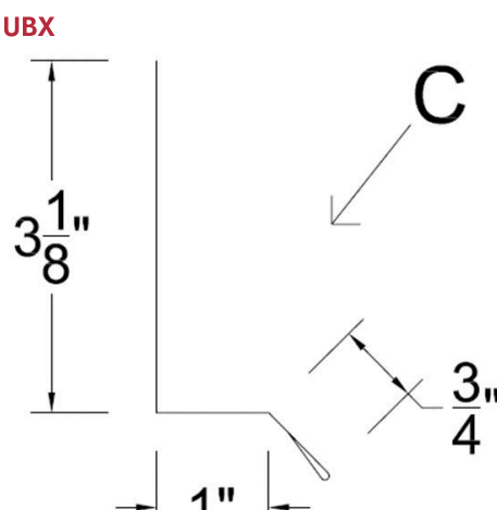
U Panel Base Trim
