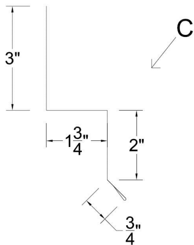
R Panel Wainscot
