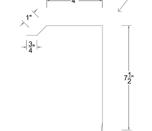
U Panel House Rake 7 1/2" Reveal
