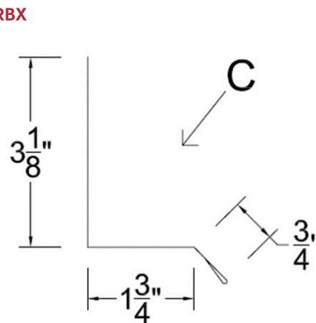
R Panel Base Trim
