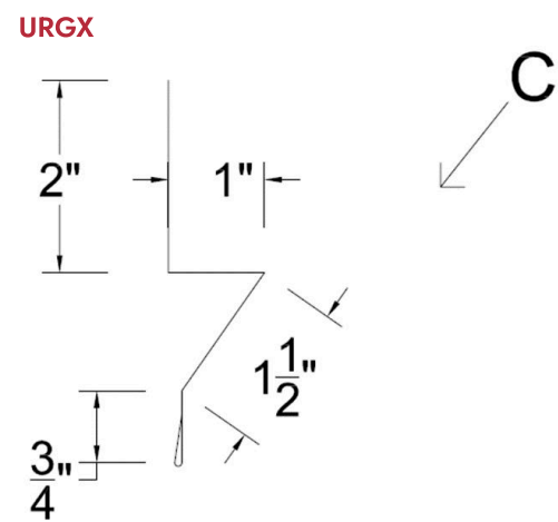
U Panel Rat Guard
