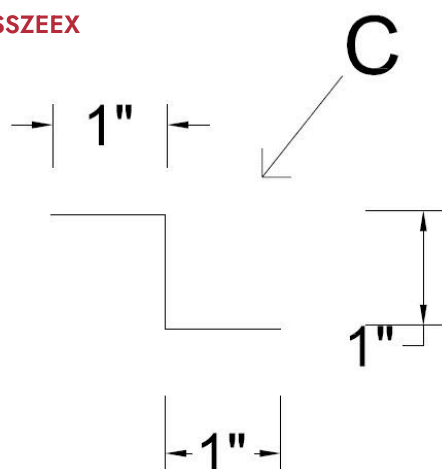
Standing Seam Zee Closure
